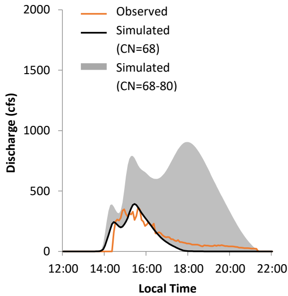
Figure F 3: Map showing the extent of storm b (top), and the comparison of observed and simulated hydrographs for the curve number loss method (bottom left) and the initial and constant loss method (bottom right).
